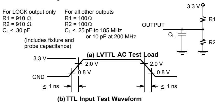
Figure 4. AC Test Loads and Waveforms
