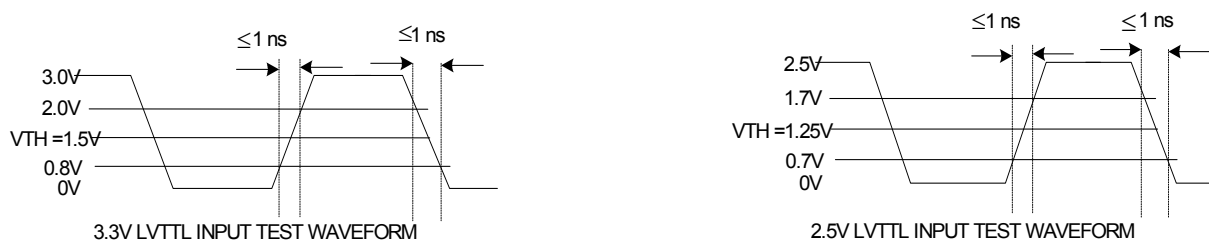
Figure 4. Test Waveforms
