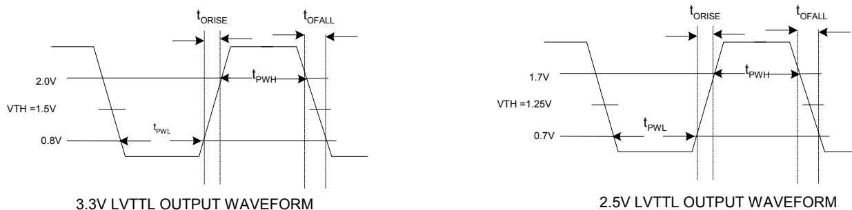
Figure 4. Test Waveforms
