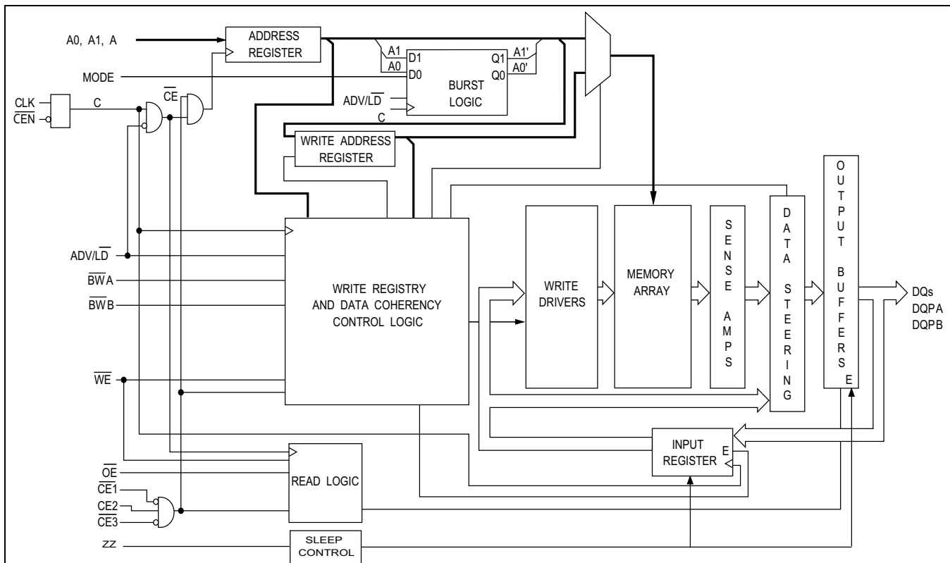
Logic Block Diagram – CY7C1473V25 (4M x 18)
