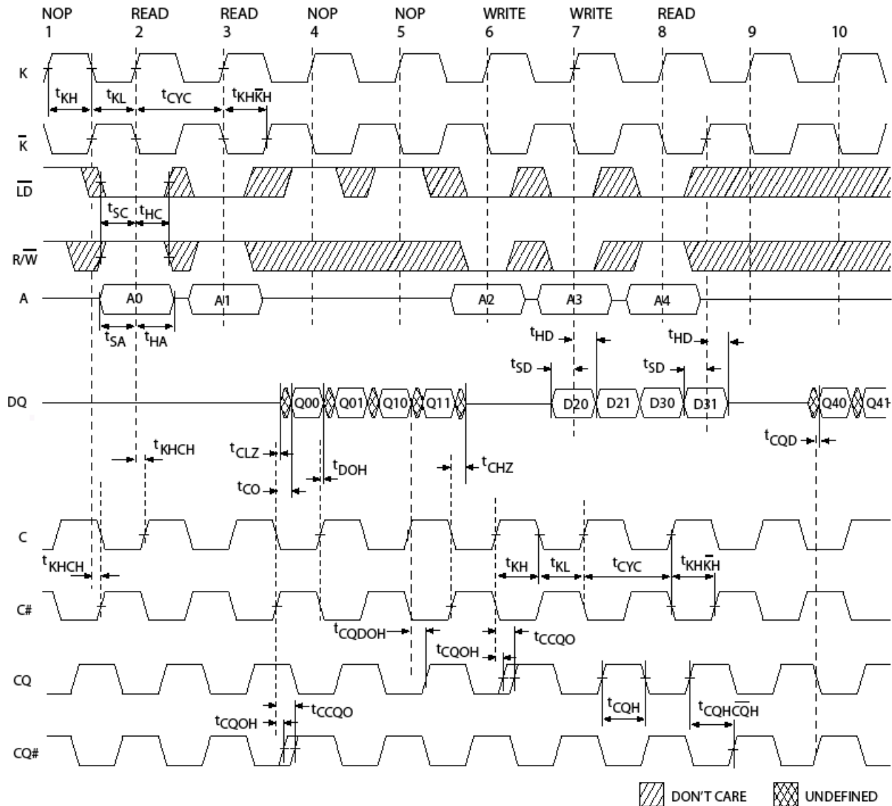
Figure 6. Read/Write/Deselect Sequence [35, 36, 37]
