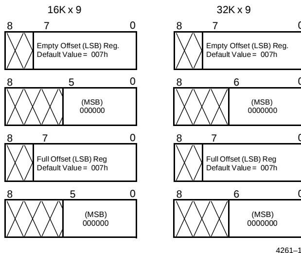
Figure 1. Offset Register Location and Default Values
