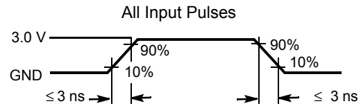
Figure 4. AC Test Loads and Waveforms (-15) [8, 9]
