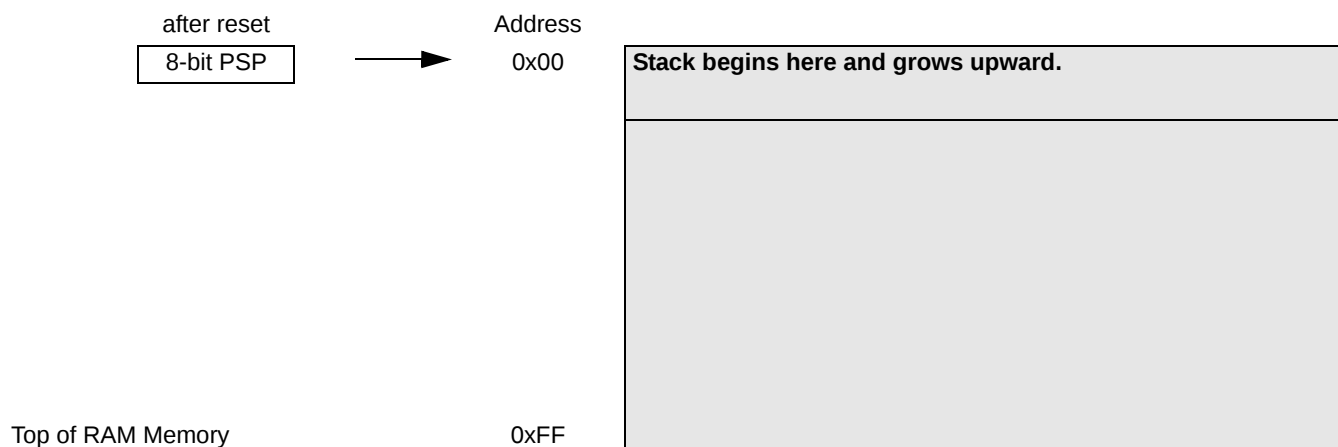
Figure 5. Data Memory Organization
