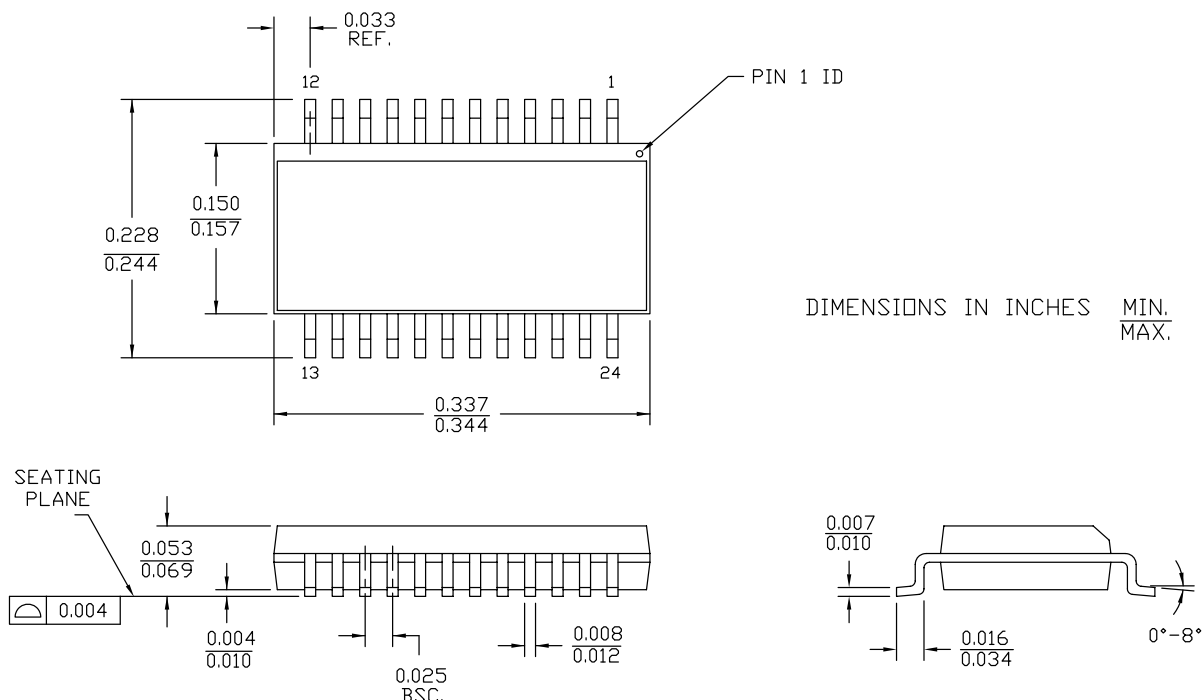
Figure 34. 24-pin QSOP (8.65 × 3.9 × 1.44 mm) O241 Package Outline, 51-85055
