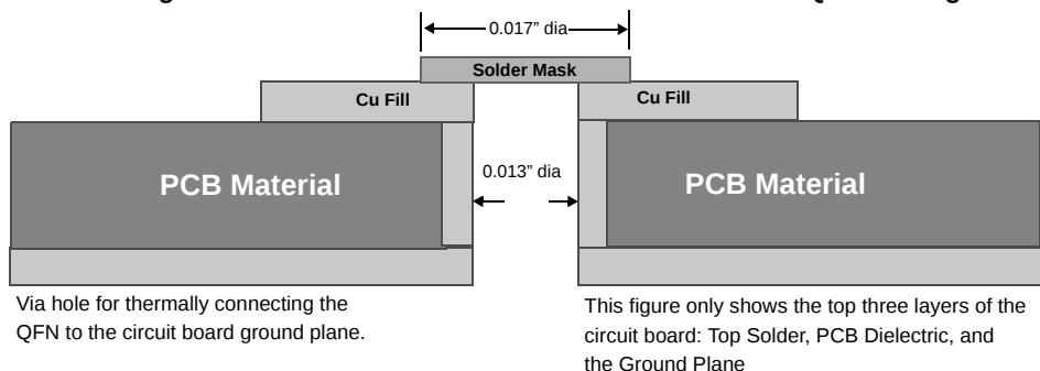
Figure 20. Cross Section of the Area Underneath the QFN Package
