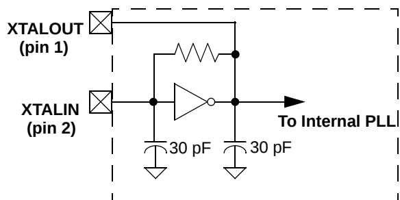
Figure 4. Clock Oscillator On-Chip Circuit
