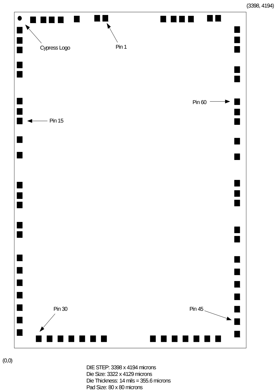
Figure 3. CY7C66113C DIE
