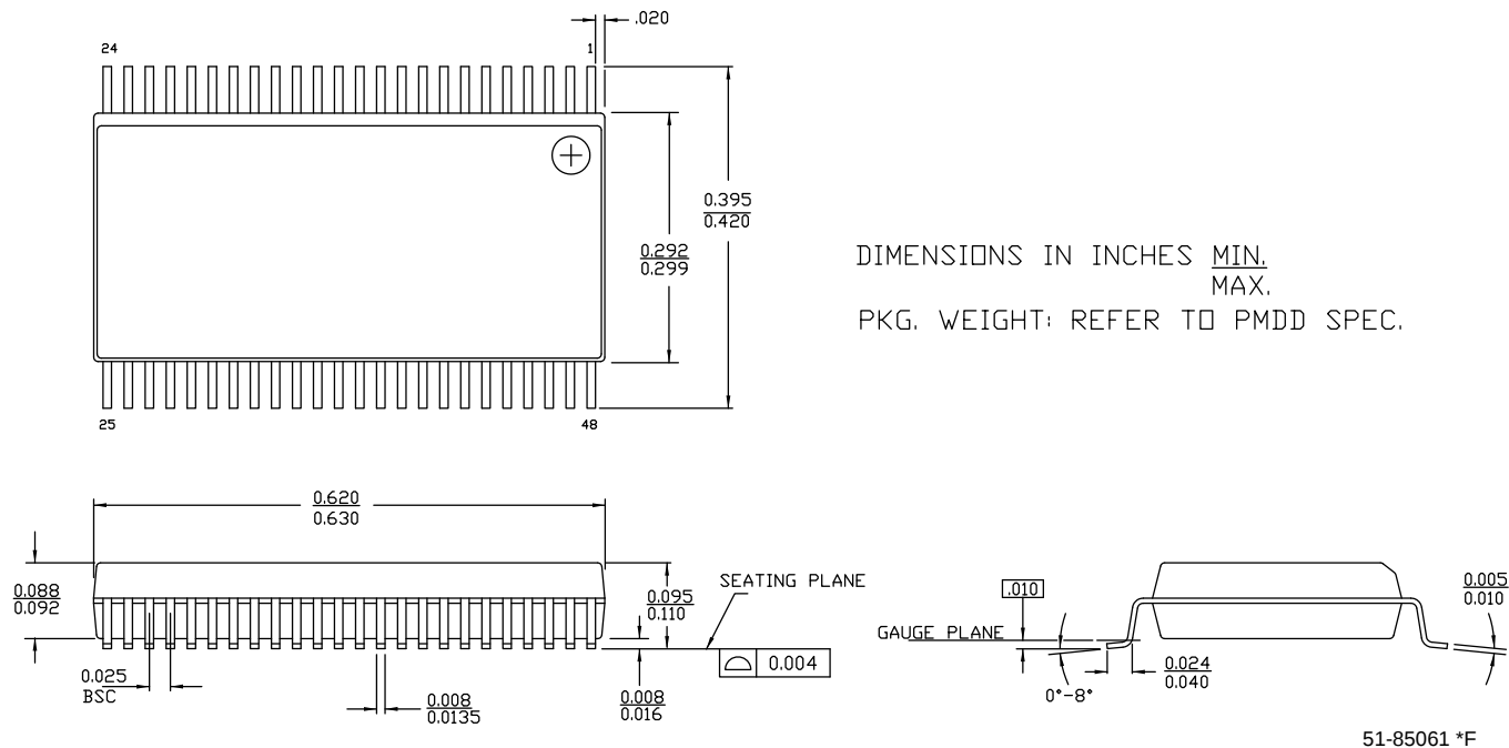
Figure 17. 48-pin Shrunk Small Outline Package O48
