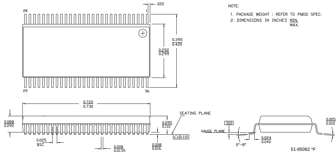
Figure 18. 56-pin Shrunk Small Outline Package O56
