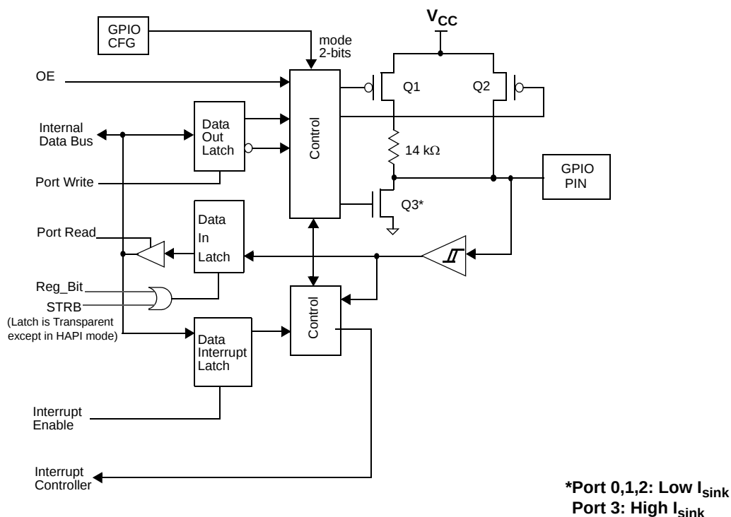
Figure 6. Block Diagram of a GPIO Pin
