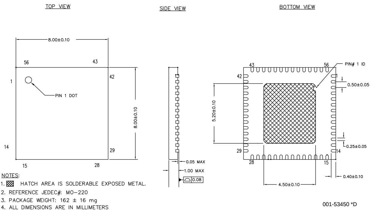
Figure 19. 56-QFN 8 × 8 × 1.0 mm EPad 4.5 × 5.2 mm
