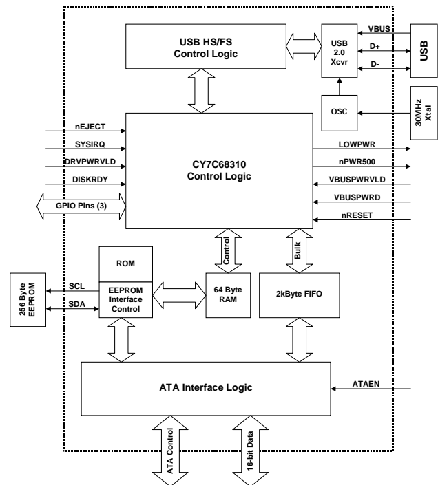
Figure 1-1. Block Diagram
