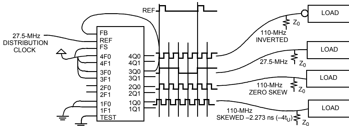
Figure 7. Multi-Function Clock Driver
