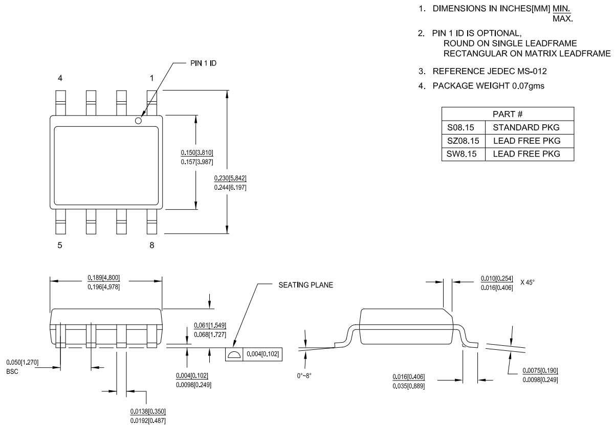
Figure 16. 8-pin SOIC (150 Mils) S08.15/SZ08.15 Package Outline, 51-85066
