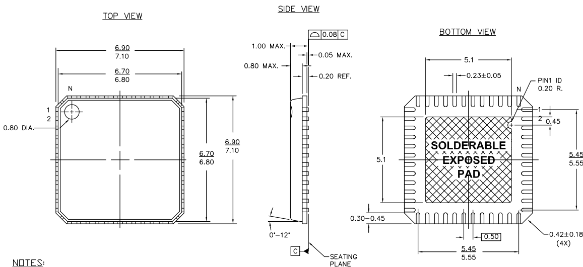
Figure 15. 48-pin (7 × 7 mm) QFN
