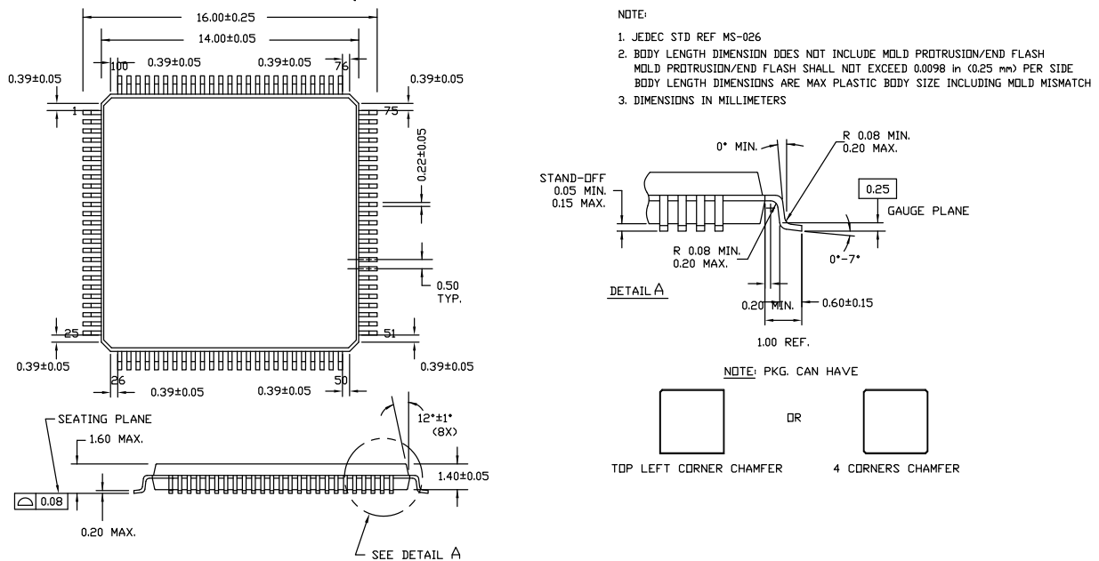
Figure 21. 100-pin TQFP (14 × 14 × 1.4 mm) A100SA Package Outline, 51-85048
