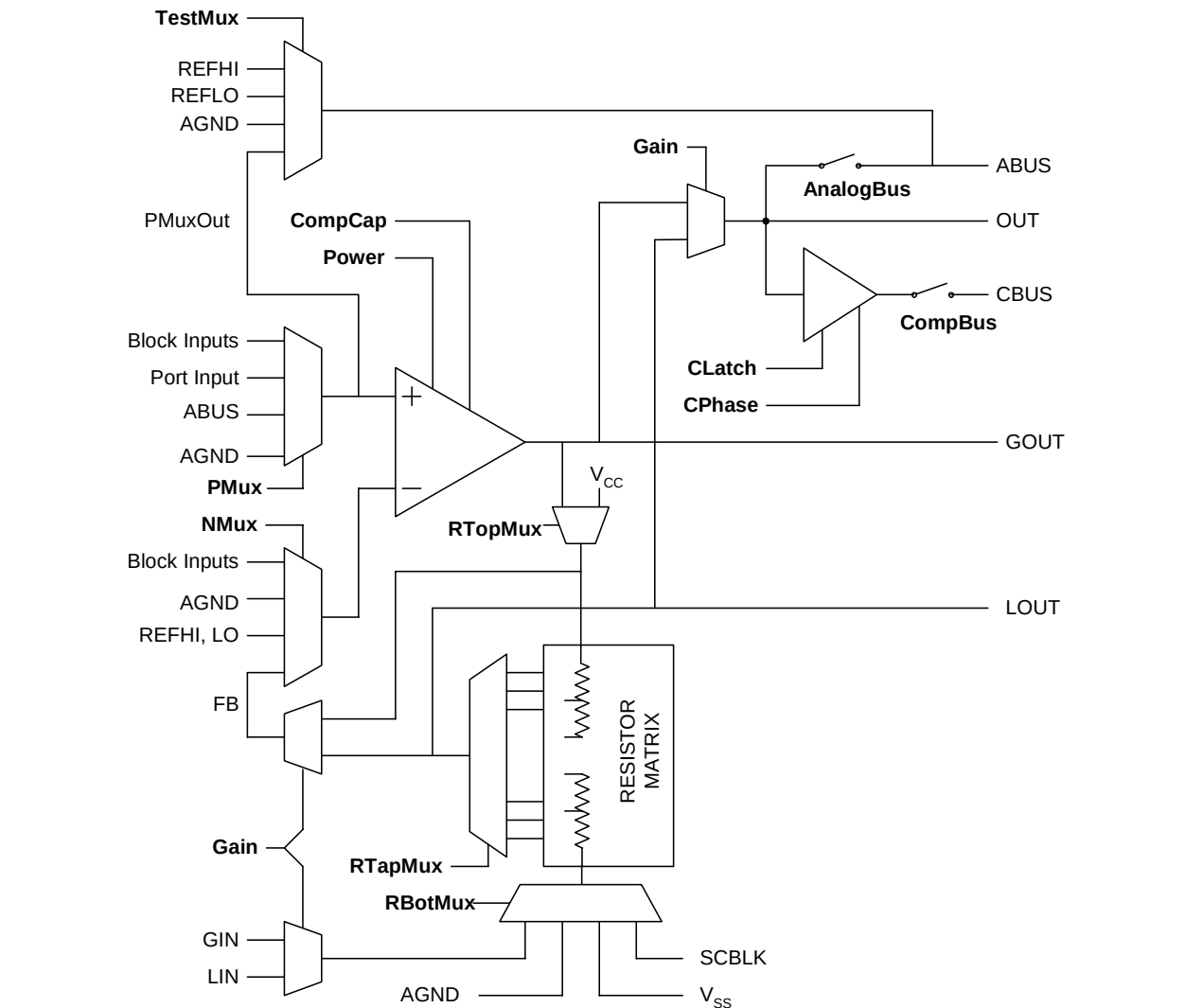
Figure 21: Analog Continuous Time PSoC Blocks
