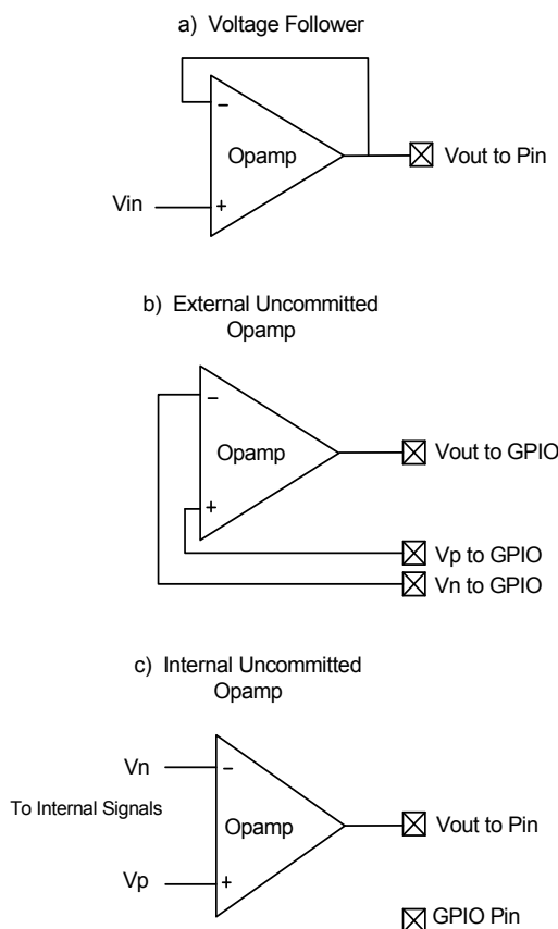
Figure 8-8. Opamp Configurations
