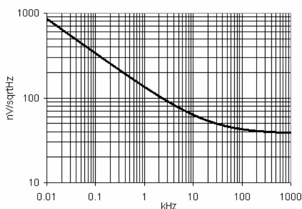
Figure 11-65. Noise vs. Frequency, V DDA = 5 V, Power Mode = High
