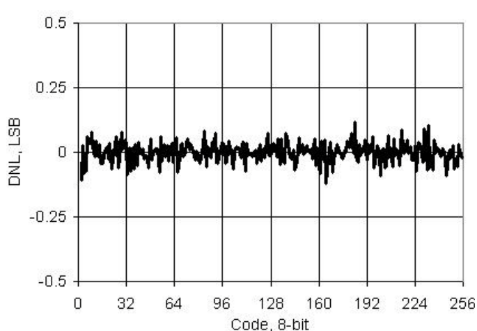
Figure 11-53. VDAC DNL vs Input Code, 1 V Mode
