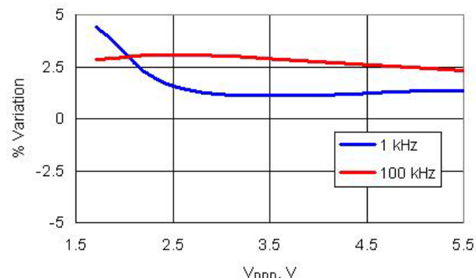
Figure 11-77. ILO Frequency Variation vs. V_{DD}
