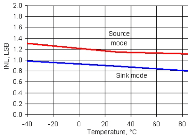
Figure 11-43. IDAC INL vs Temperature, Range = 255 \mu A, Fast Mode
