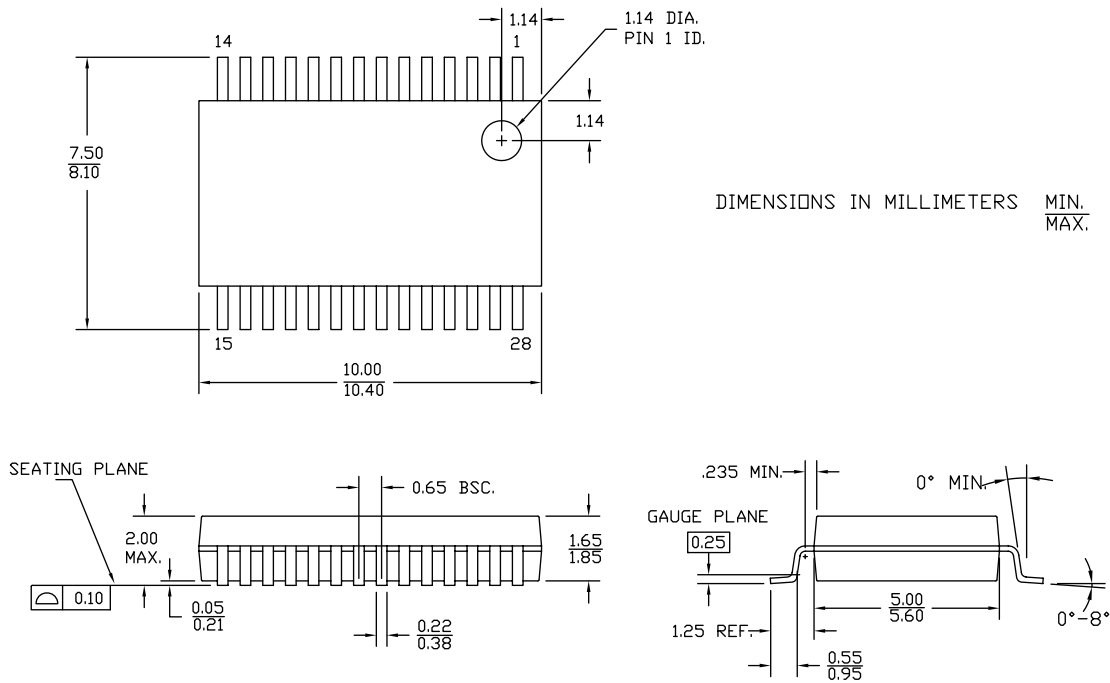
Figure 21. 28-Pin (210-Mil) SSOP
