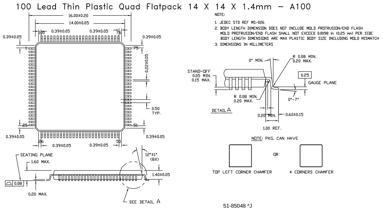
Figure 24. 100-Pin TQFP
