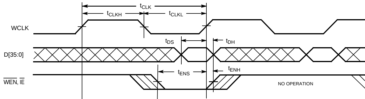
Figure 6. Write Cycle Timing
