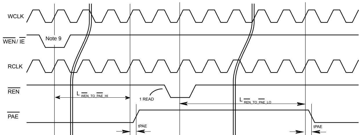
Figure 20. \overline{\text{PAE}} Assertion and Deassertion
