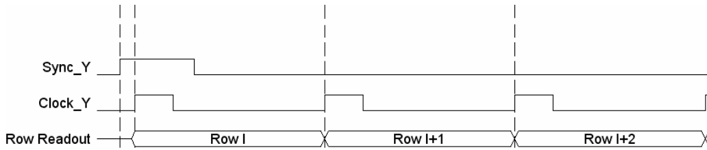
Figure 14. Timing of y Shift Register
