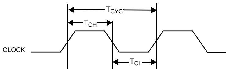
Figure 20. Clock Timing
