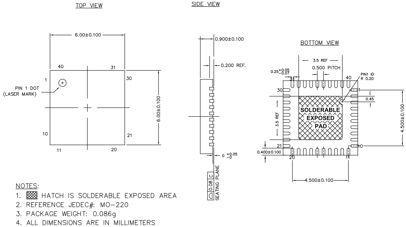
Figure 31. 40-pin QFN (6 × 6 × 1.0 mm) LT40B (3.5 × 3.5 mm) E-Pad (Sawn) Package Outline, 001-13190
