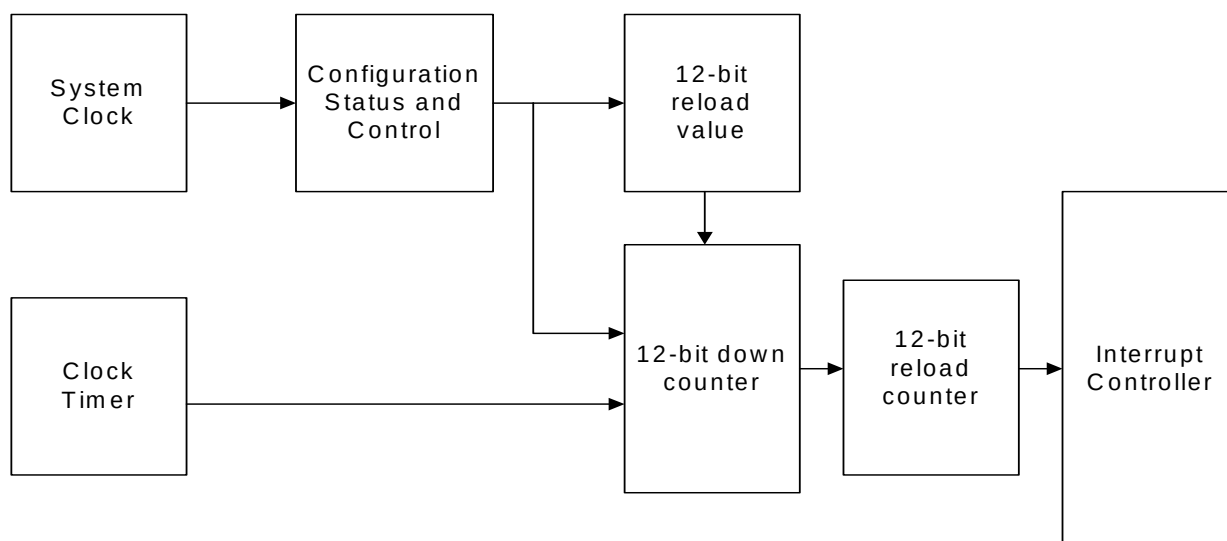
Figure 9. Programmable Interval Timer Block Diagram
