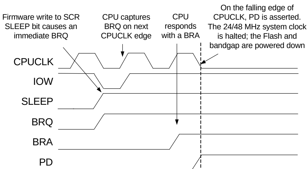
Figure 11. Sleep Timing
