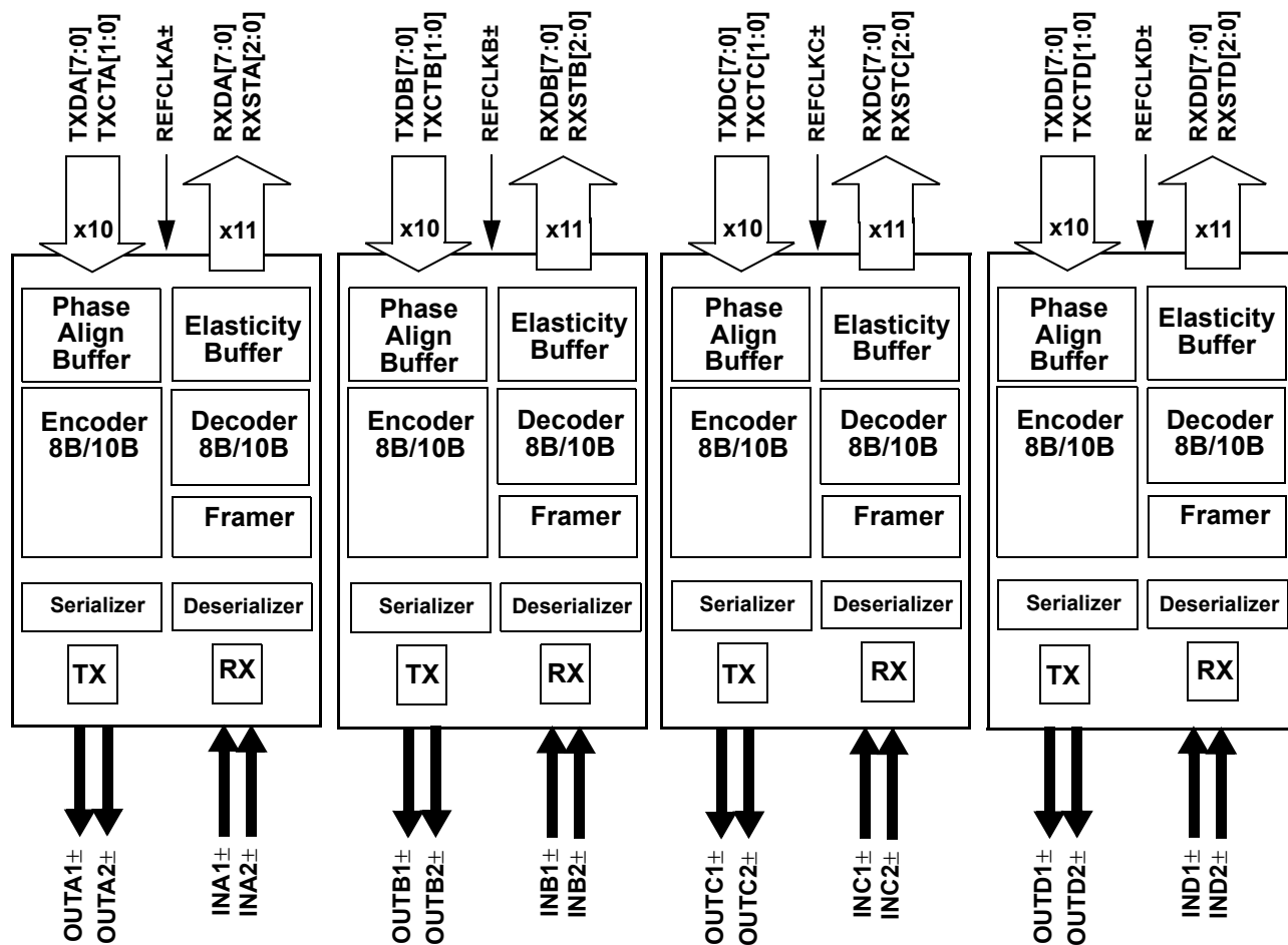
CYP(V)15G0403DXB Transceiver Logic Block Diagram
