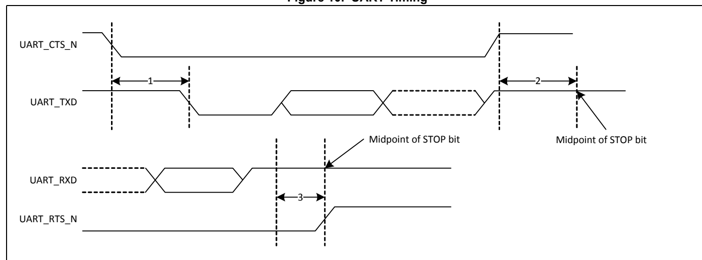
Figure 10. UART Timing
