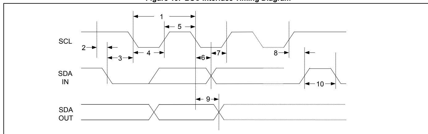
Figure 19. BSC Interface Timing Diagram
