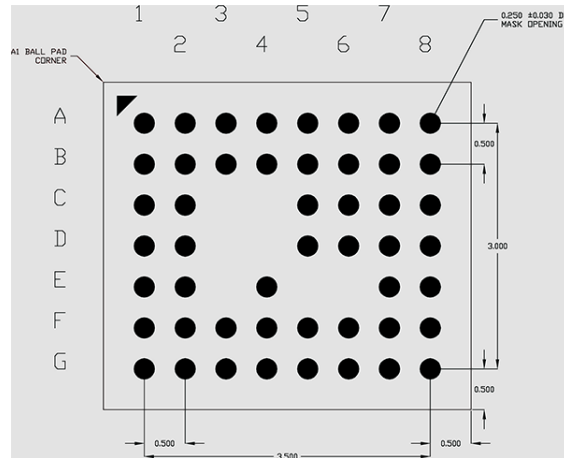
Figure 6. 4.5 mm x 4 mm x 0.8 mm (FcBGA) Array
