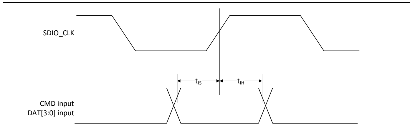
Figure 27. SDIO Bus Input Timing (SDR Modes)
