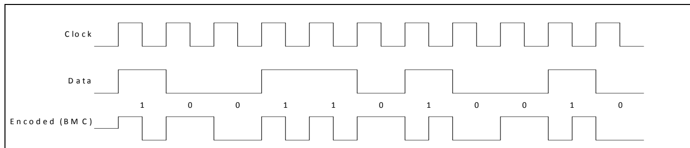
Figure 29. S/PDIF Interface Timing
