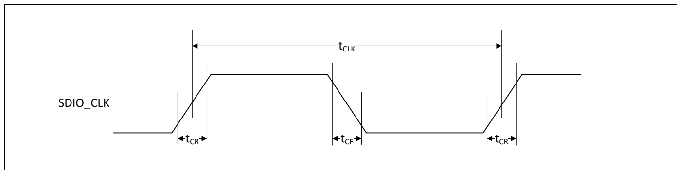
Figure 26. SDIO Clock Timing (SDR Modes)
