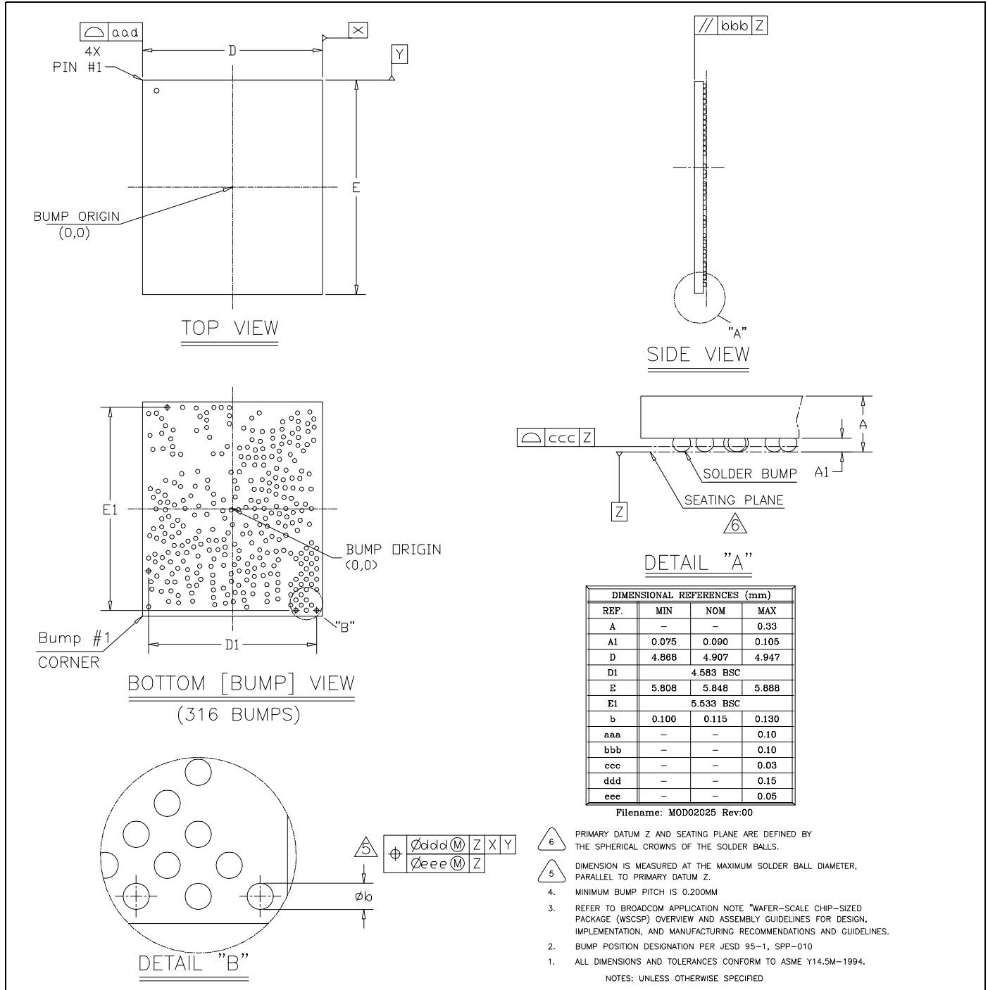
Figure 41. WLCSP Package
