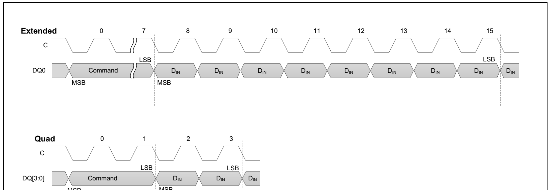
Figure 32. SPI Flash Write-Register Timing
