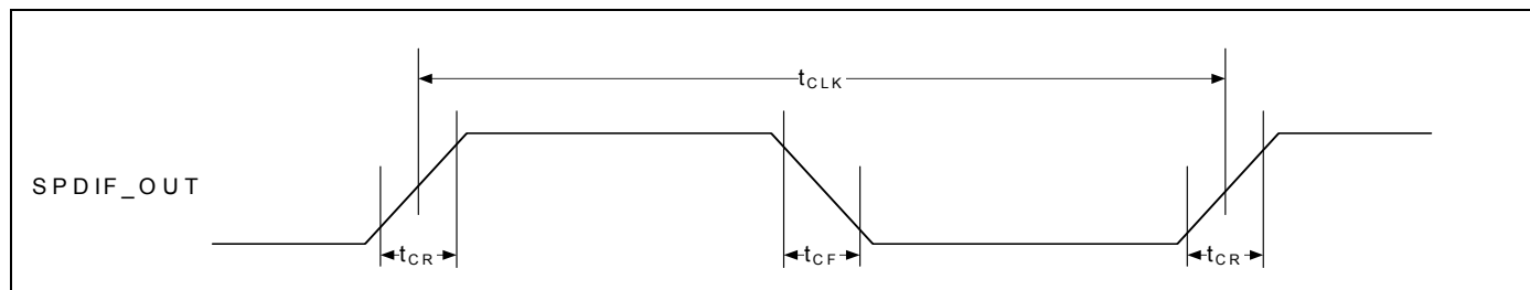
Figure 30. S/PDIF Data Output Timing
