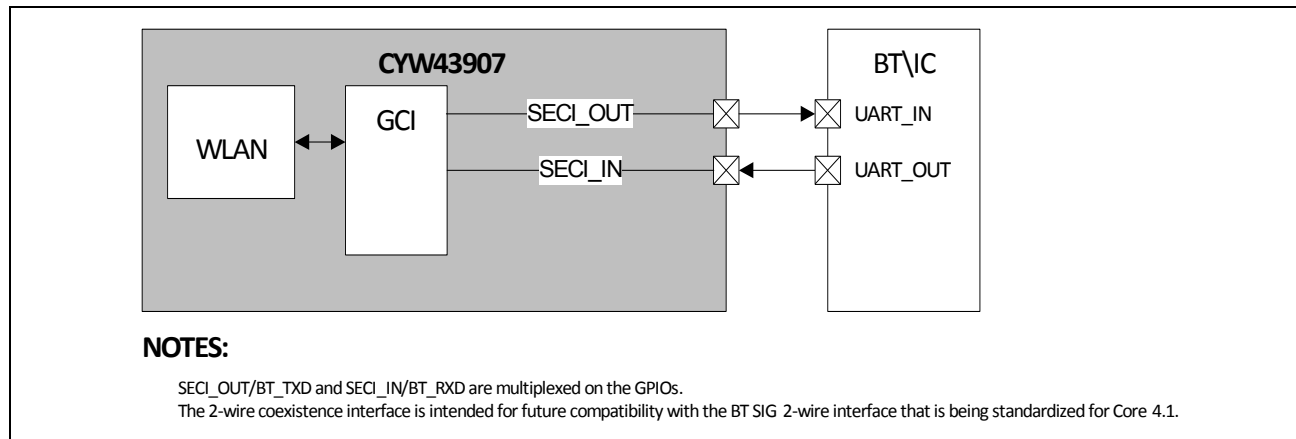
Figure 11. Cypress 2-Wire External Coexistence Interface
