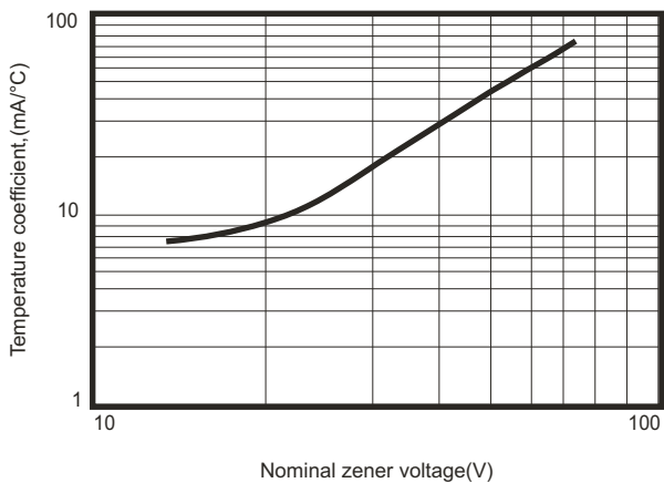
Fig.3 Temperature coefficients
