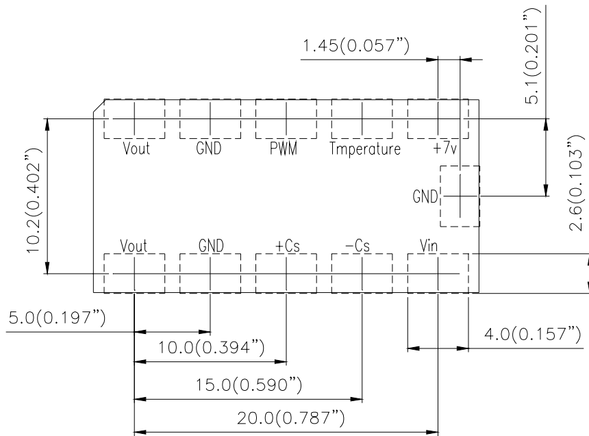
RECOMMENDED P.W.B PAD LAYOUT
