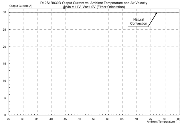
Figure 19: Output current vs. ambient temperature and air velocity @ V in =11V, V out =1.0V (Either Orientation)
