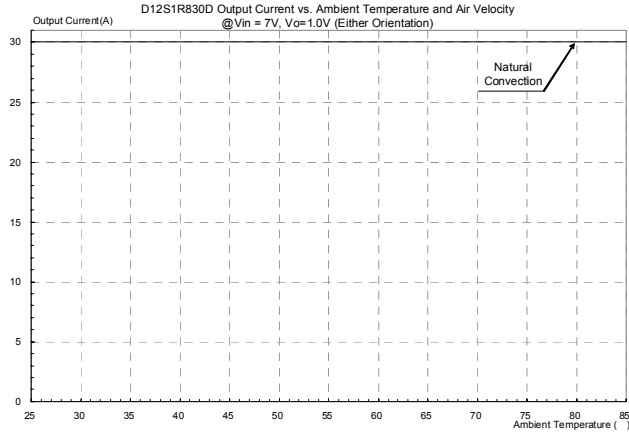
Figure 17: Output current vs. ambient temperature and air velocity @ V in =7V, V out =1.0V (Either Orientation)
