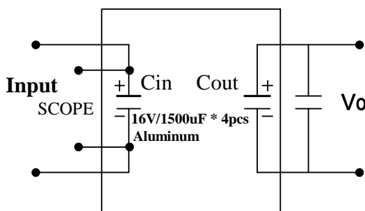
Figure 13: Peak-peak Input ripple & noise measurement test setup
