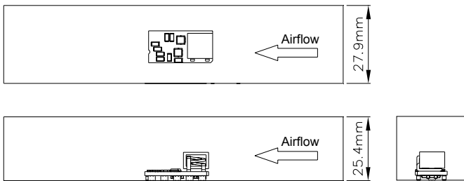
Figure 14: Wind Tunnel Test Setup
