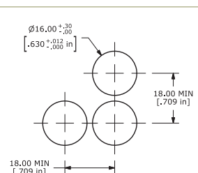
PANEL MOUNTING
