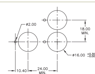
PANEL MOUNTING
