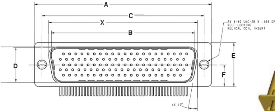
Plug - Pin
