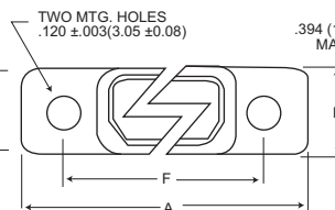
Pigtail termination
