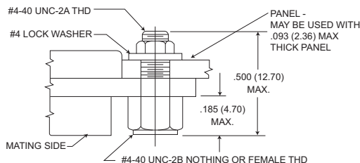
Jackpost - (P)
