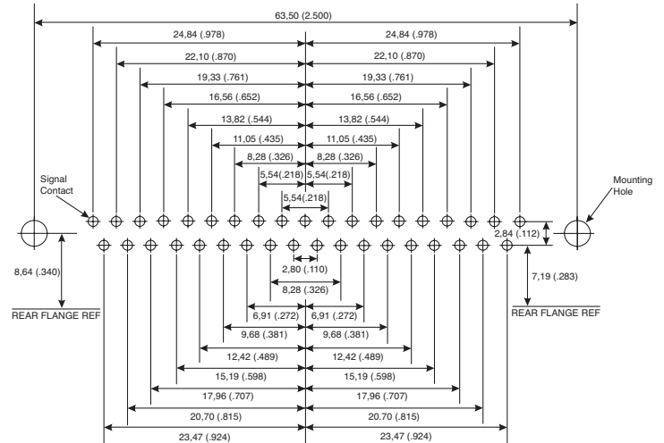
37 Contacts
