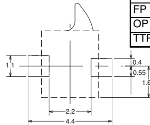
PCB mounting land Dimension (Reference) (View from switch top)
