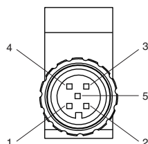
Pin arrangement of D40A connector type
