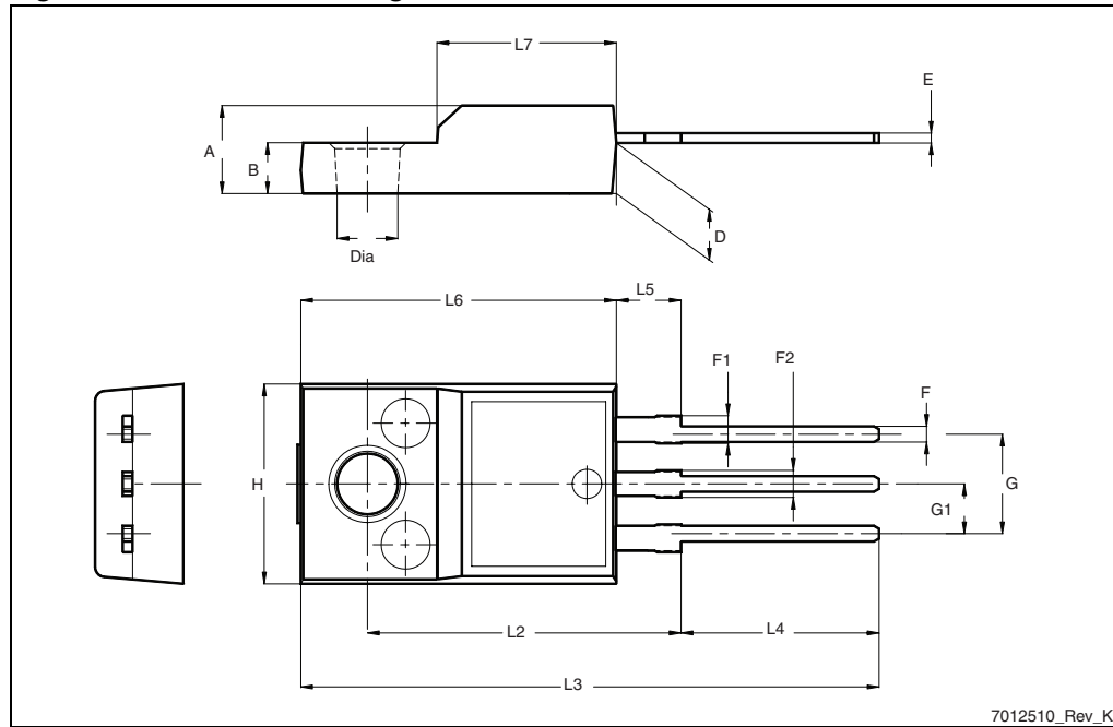
Figure 6. TO-220FP drawing
