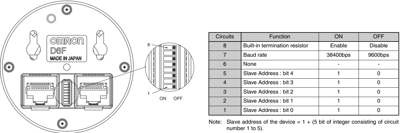
Fig. 3. DIP Switches
