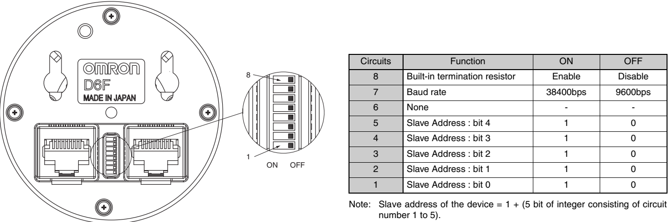
Fig. 3. DIP Switches
