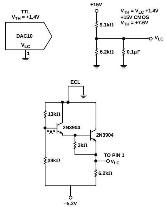
Figure 17. Interfacing with Various Logic Families
