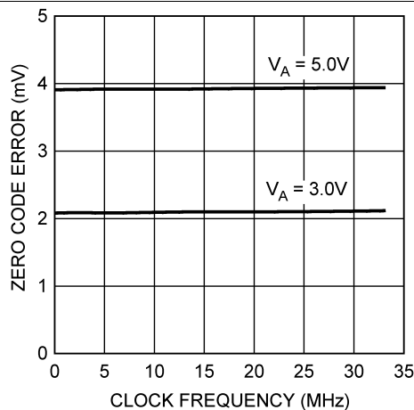
Figure 22. Zero Code Error vs. f_{\text{SCLK}}
