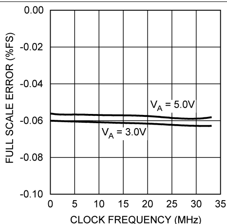
Figure 25. Full-Scale Error vs. f_{\text{SCLK}}
