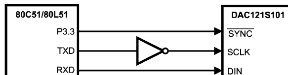
FIGURE 6. 80C51/80L51 Interface
