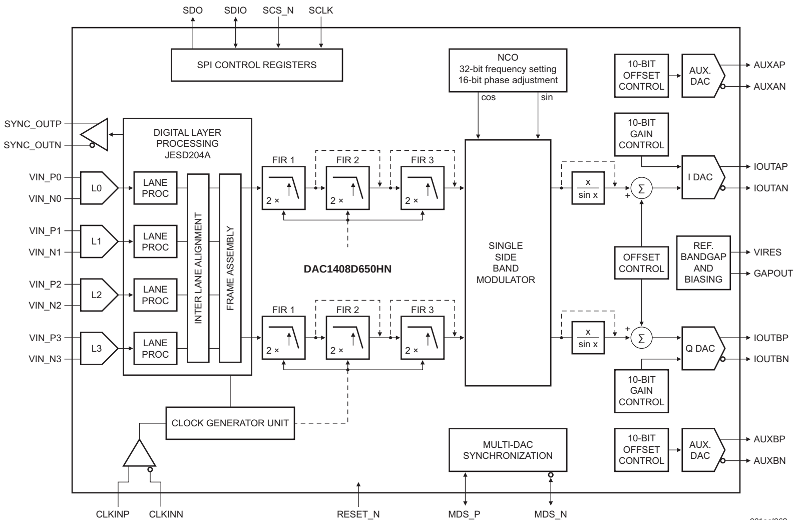
Fig 1. Block diagram
