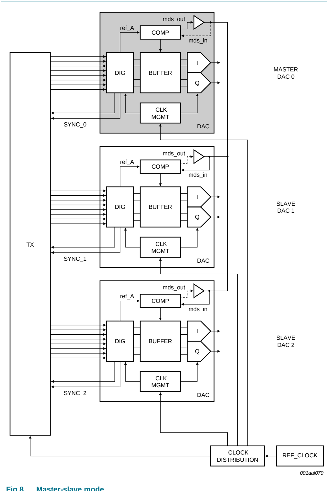
Fig 8. Master-slave mode
