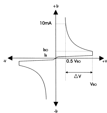
DIAGRAM 1: Current-voltage characteristics
