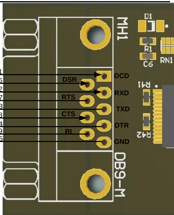
Figure 3.2 – DB9-USB Male Connection illustration
