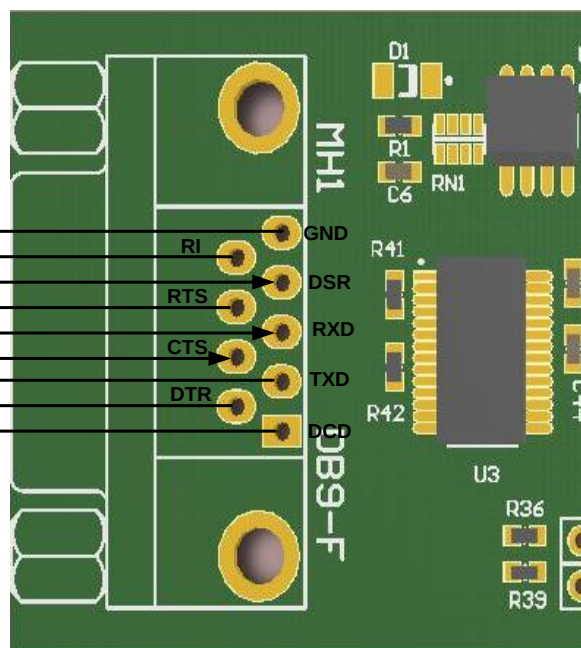
Figure 3.3 – DB9-USB Female Connection illustration
