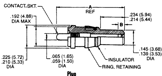
Plug
