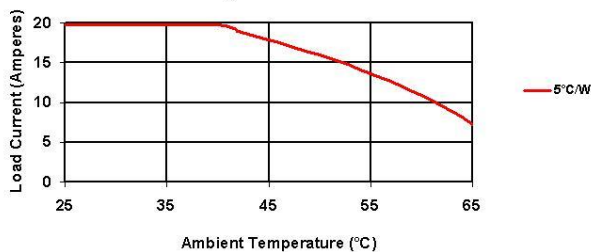
Derating Curve: DC100A10
