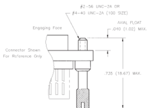
Standard Jackscrew
