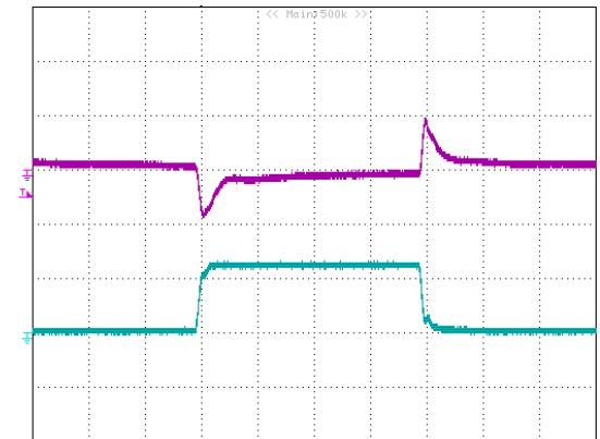
Figure 22: Typical transient response to step load change at 2.5\text{A}/\mu\text{s} from 0% to 50% to 0% of I_o , max at 5V_{in} , 3.3V_{out} (100uS/div) ( C_{out} = 47\mu\text{F} ceramic). top trace: V_{out} , 0.2V/div; bottom trace: I_{out} : 5A/div.
