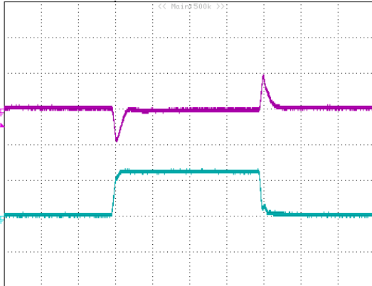
Figure 19: Typical transient response to step load change at 2.5\text{A}/\mu\text{s} from 0% to 50% to 0% of I_o , max at 5V_{in} , 0.6V_{out} (100uS/div) ( C_{out} = 47\mu\text{F} ceramic). top trace: V_{out} , 0.2V/div; bottom trace: I_{out} : 5A/div.
