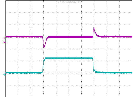
Figure 20: Typical transient response to step load change at 2.5\text{A}/\mu\text{s} from 0% to 50% to 0% of I_o , max at 5V_{in} , 1.2V_{out} (100uS/div) ( C_{out} = 47\mu\text{F} ceramic). top trace: V_{out} , 0.2V/div; bottom trace: I_{out} : 5A/div.
