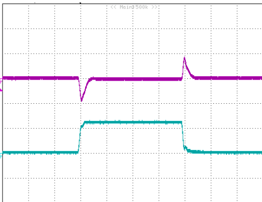
Figure 21: Typical transient response to step load change at 2.5\text{A}/\mu\text{s} from 0% to 50% to 0% of I_o , max at 5V_{in} , 1.8V_{out} (100uS/div) ( C_{out} = 47\mu\text{F} ceramic). top trace: V_{out} , 0.2V/div; bottom trace: I_{out} : 5A/div.
