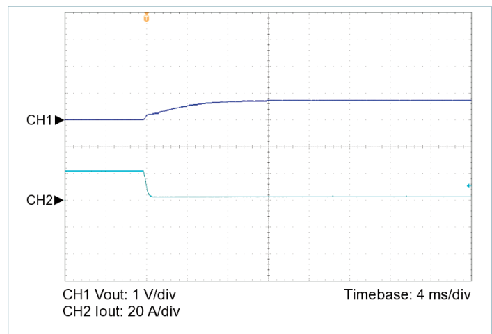
Figure 7 — 100% to 10% load transient response, V_{IN} = 24\text{ V} , nominal trim, C_{OUT\_EXT} = 680\text{ }\mu\text{F}
