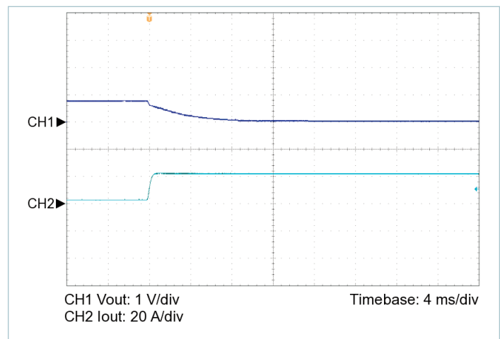
Figure 8 — 10% to 100% load transient response, V_{IN} = 24\text{ V} , nominal trim, C_{OUT\_EXT} = 680\text{ }\mu\text{F}
