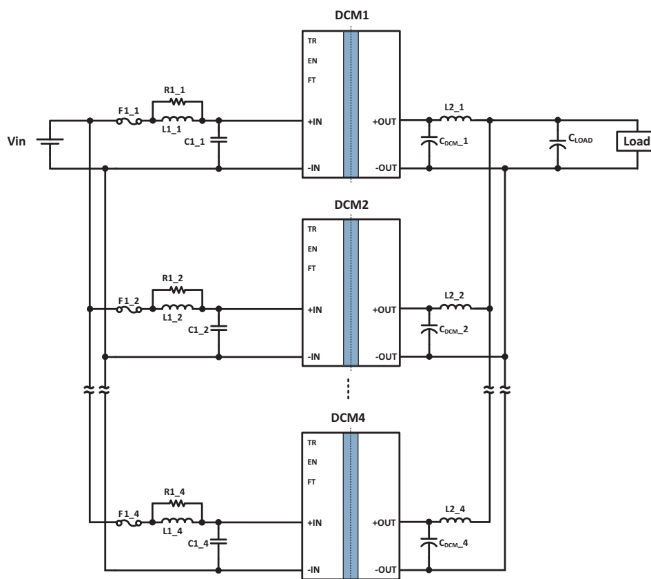
Typical Application 1: DCM48AP480x320A50 in an array of four units
