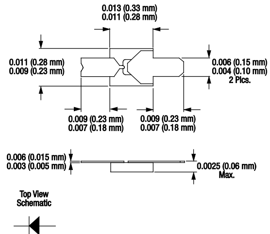
Figure 11. 491-006 Package Dimensions
