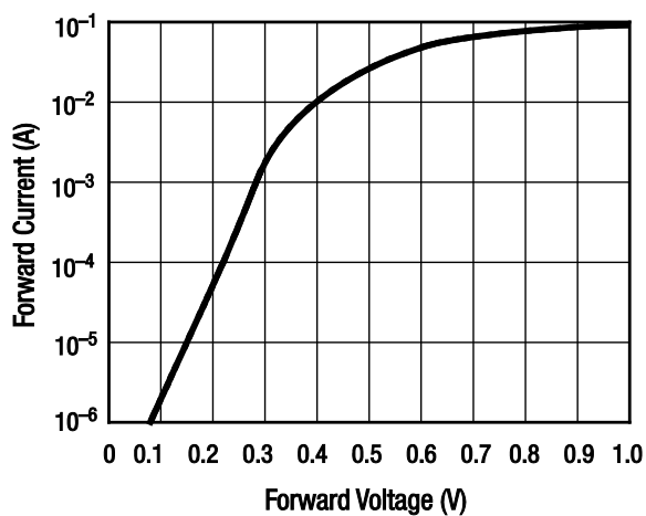
Figure 1. CDF7621-000
