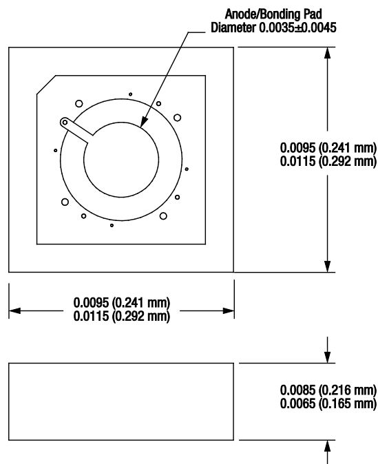
Figure 13. 571-011 Package Dimensions
