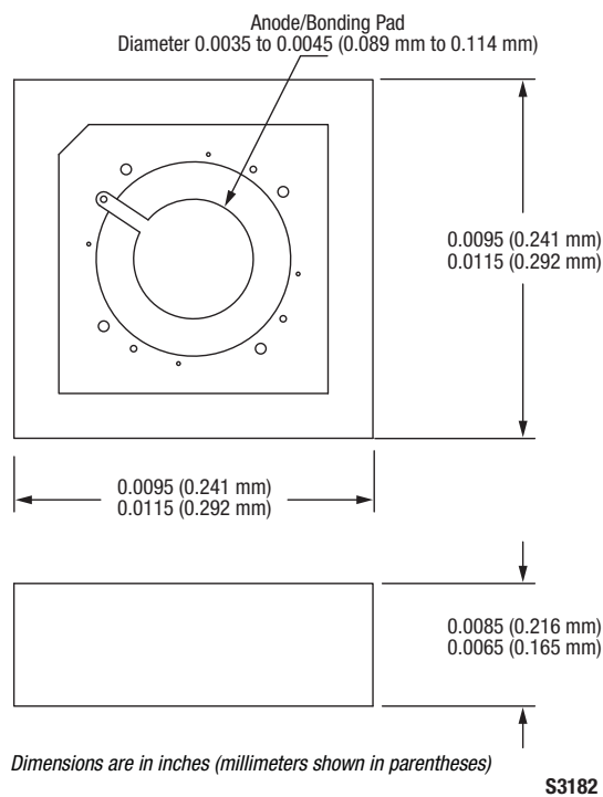
Figure 13. 571-011 Package Dimensions
