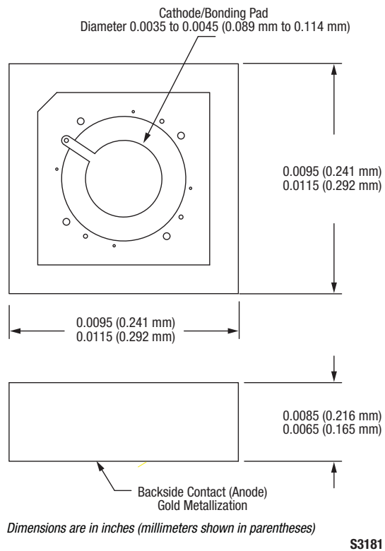
Figure 12. 571-006 Package Dimensions
