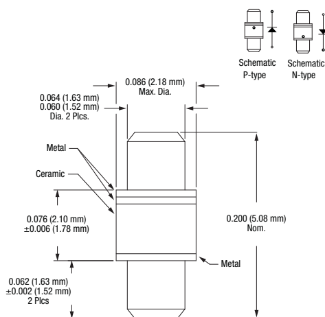
Figure 7. -207 Package Dimensions
