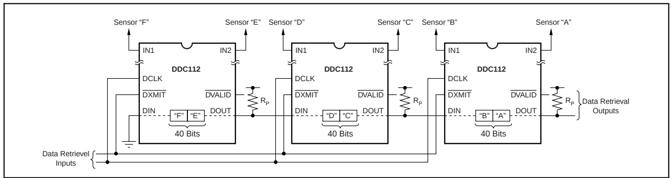
FIGURE 20. Daisy-Chained DDC112's.
