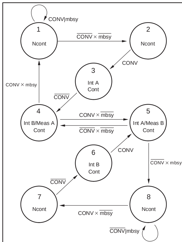
Figure 10. State Diagram
