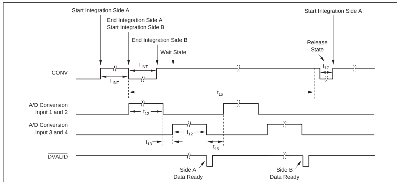
Figure 14. Conversion Detail for the Internal Operation of the Non-Continuous Mode with Side A Integrated First
