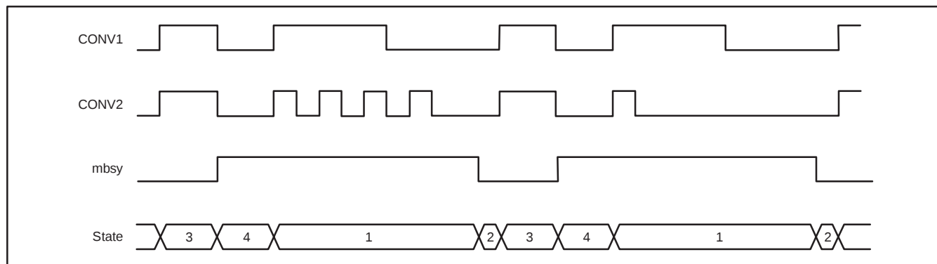
Figure 16. Equivalent CONV Signals in the Non-Continuous Mode
