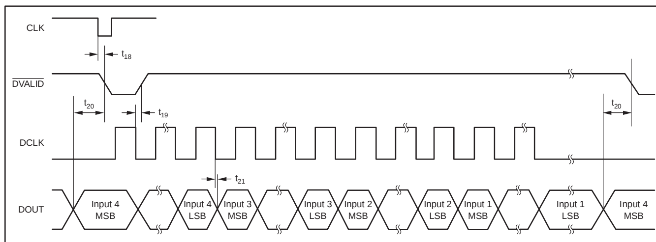
Figure 21. Digital Interface Timing Diagram for Data Retrieval From a Single DDC114
