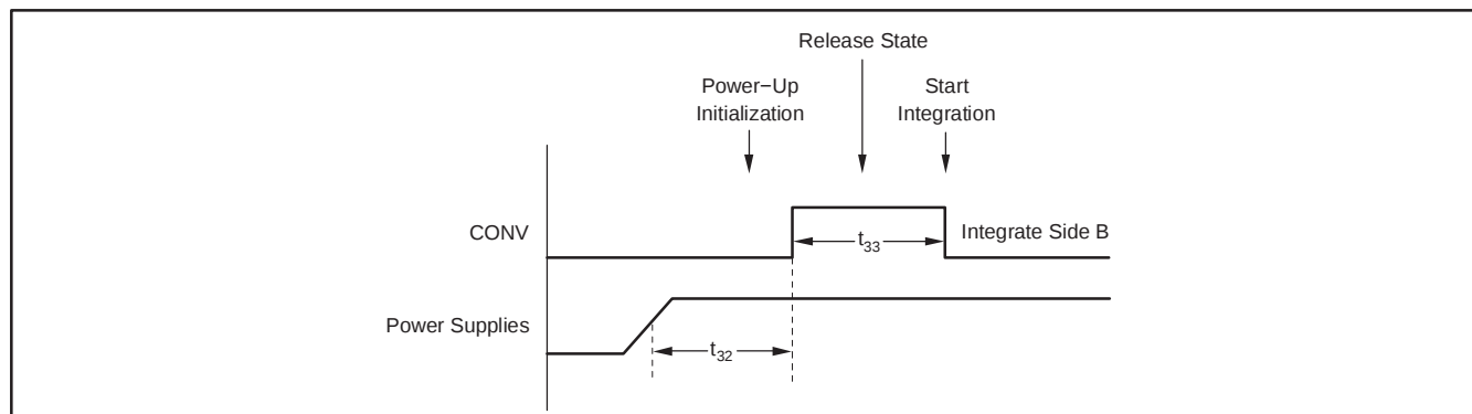
Figure 27. Timing Diagram at Power-Up of the DDC114
