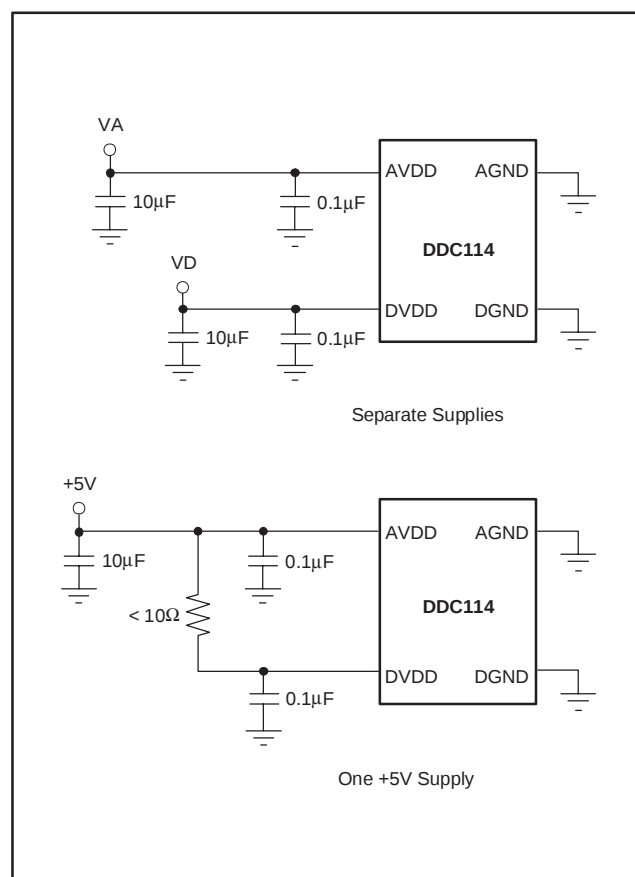
Figure 28. Power-Supply Connection Options
