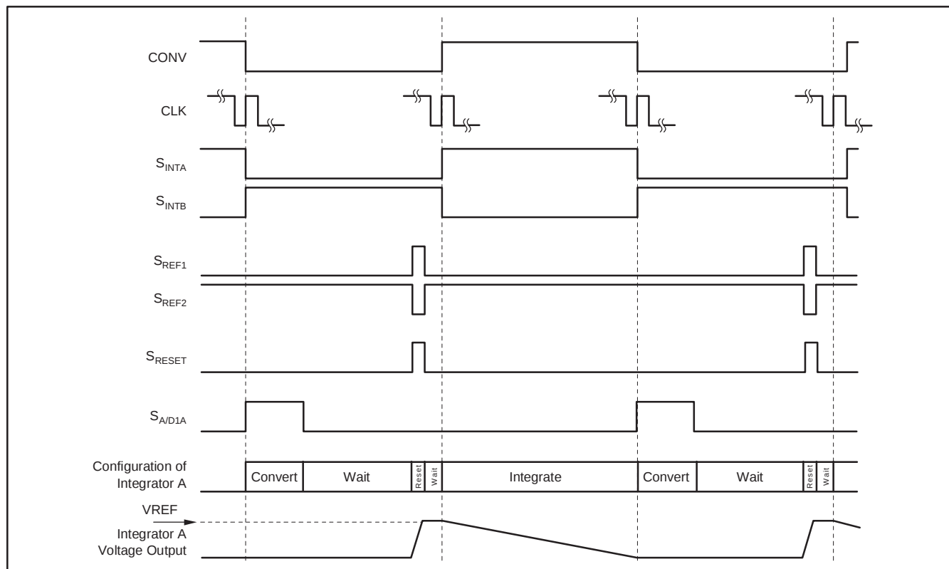
Figure 4. Basic Integration Timing Diagram (as Illustrated in Figure 3)
