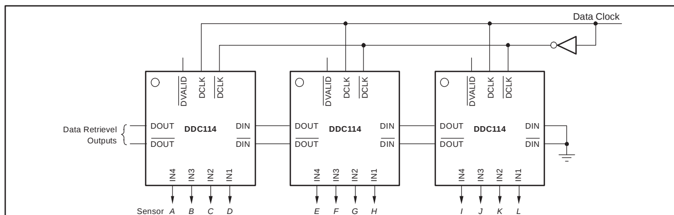
Figure 20. Daisy-Chained DDC114s
