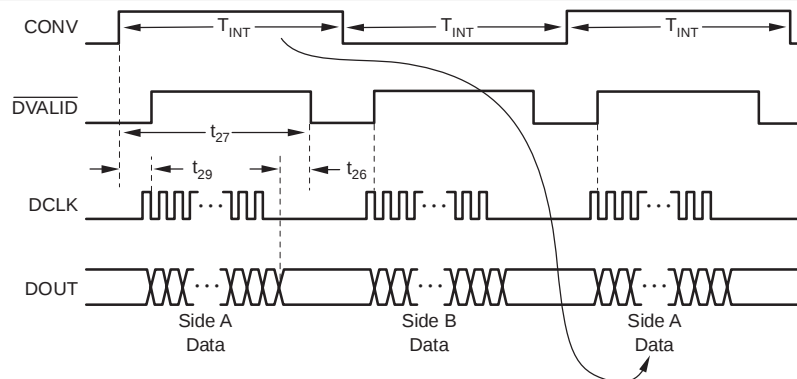
Figure 23. Readback Before CONV Toggles
