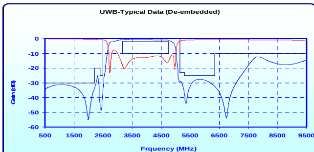
[Frequency characteristic ]
