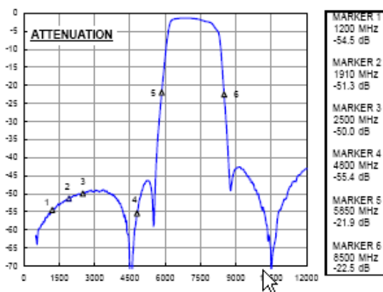
[Frequency characteristic ]
