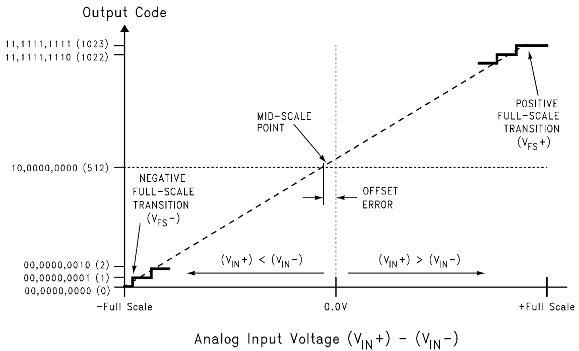
FIGURE 2. Input vs. Output Transfer Characteristic
